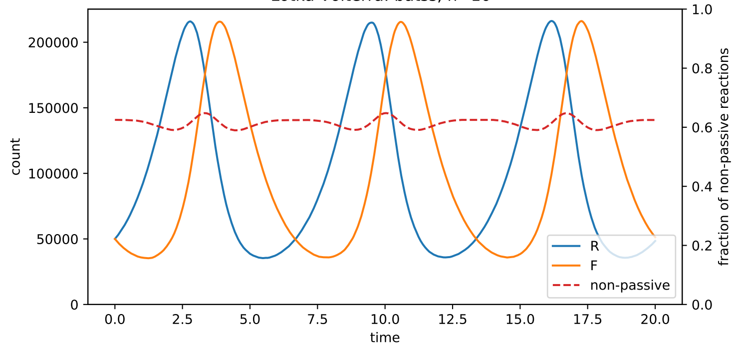
Lotka Volterra: batss, n=10^5
